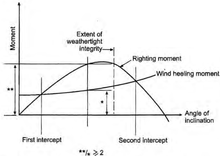
Figure 2.6-1 – Righting moment and wind heeling moment curves
