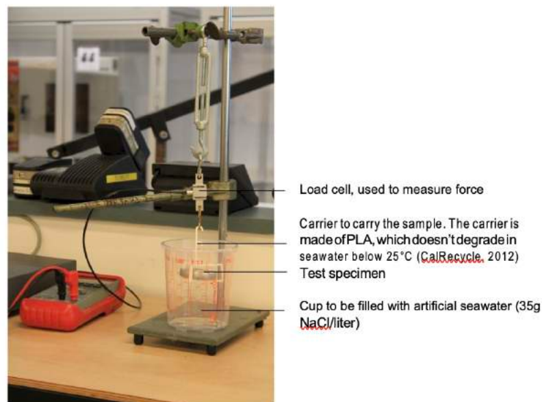
Figure 2. test set-up
